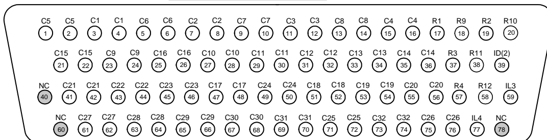
78-Pin D-Sub Male Connector Bank 1
