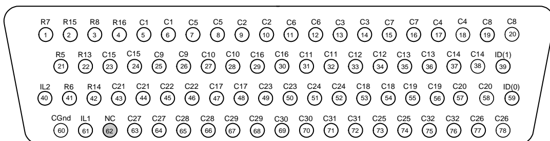
78-Pin D-Sub Male Connector Bank 2
